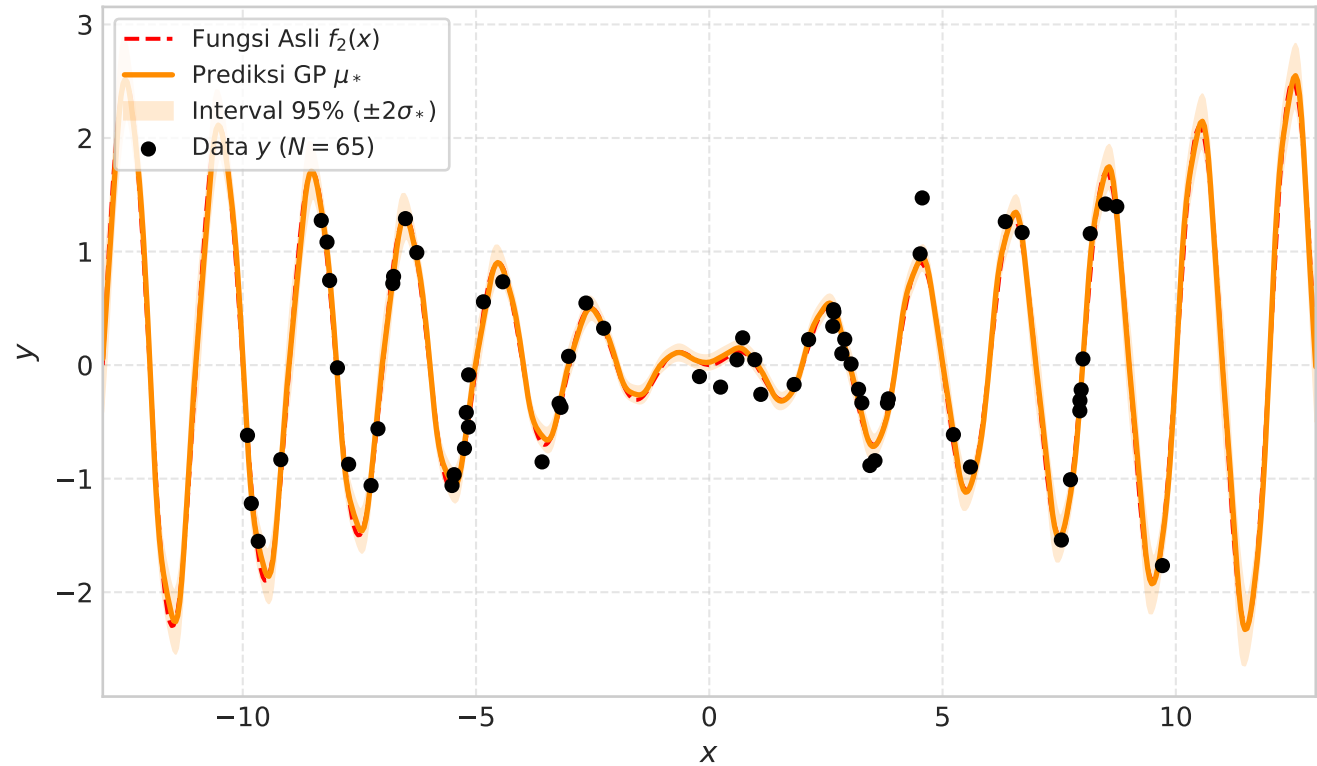
(b) Perkalian: k_{\text{Lin}} \times k_{\text{Per}}
